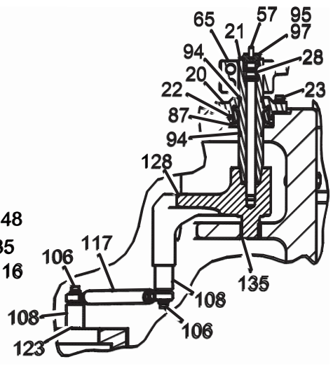
SECTION M-M
