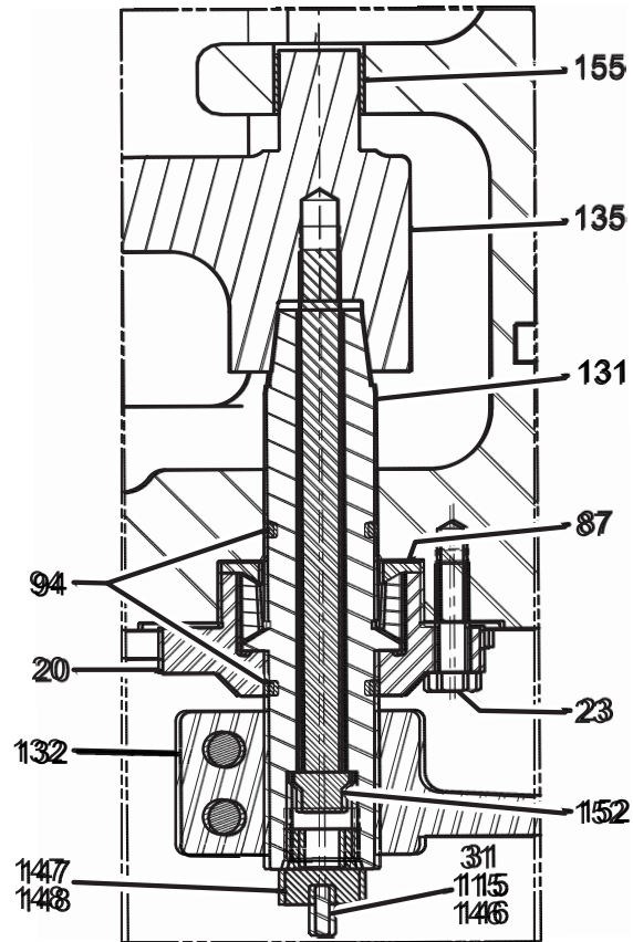
FIGURE 28 - YD COMPRESSOR COMPONENTS (J3/J4/J5)
