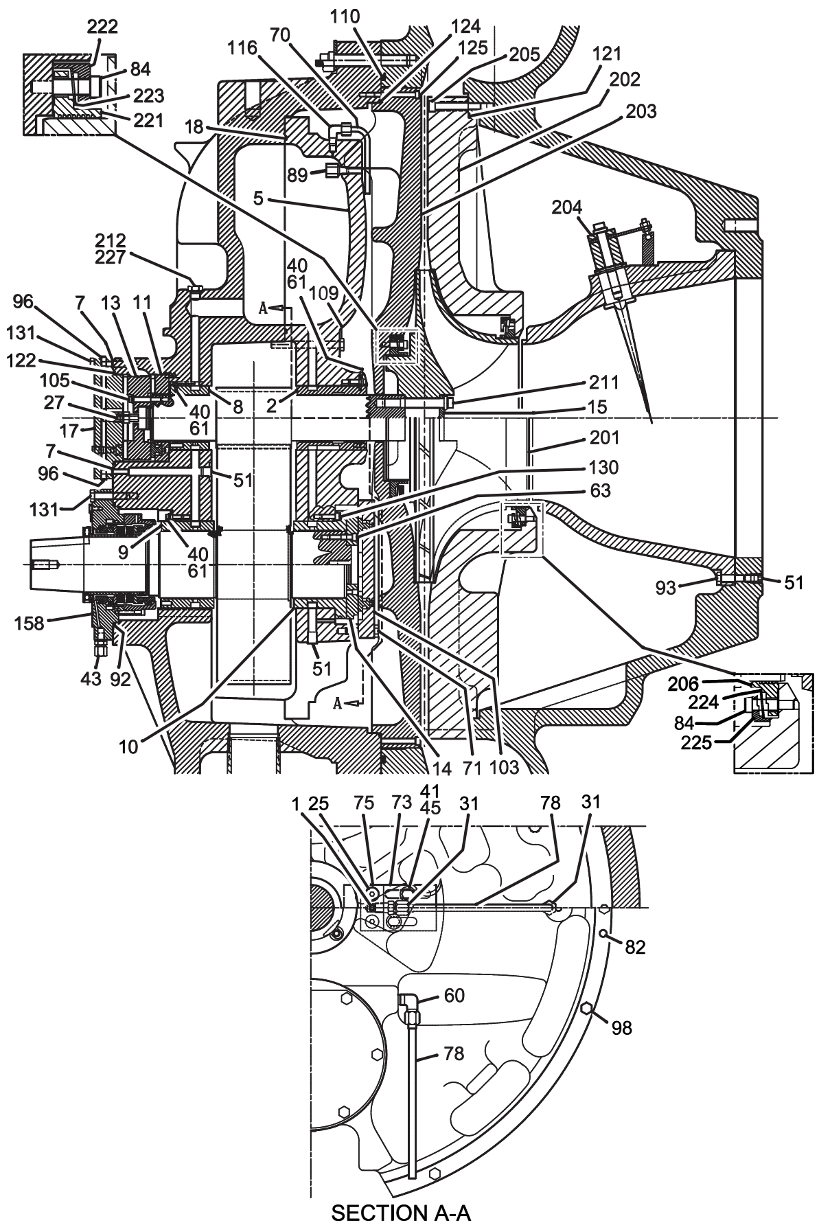
FIGURE 23 - YD COMPRESSOR COMPONENTS (J3/J4/J5)
