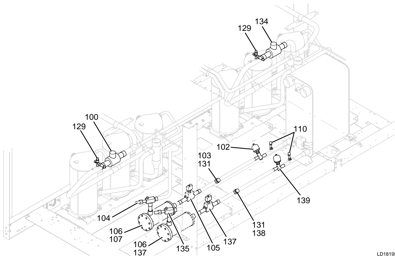
FIGURE 14 - SYSTEM PIPING (QTC3085T, QTC3110T)
