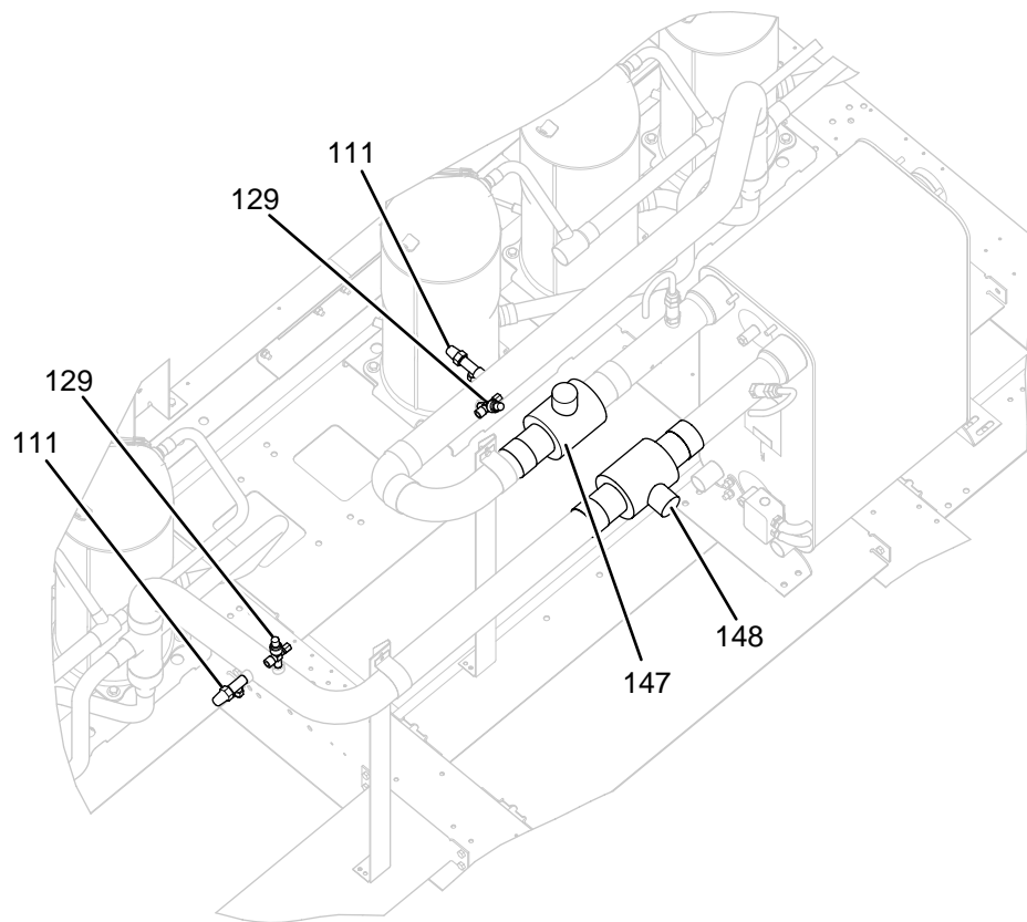
FIGURE 13 - SYSTEM PIPING (QTC3085T, QTC3110T)
