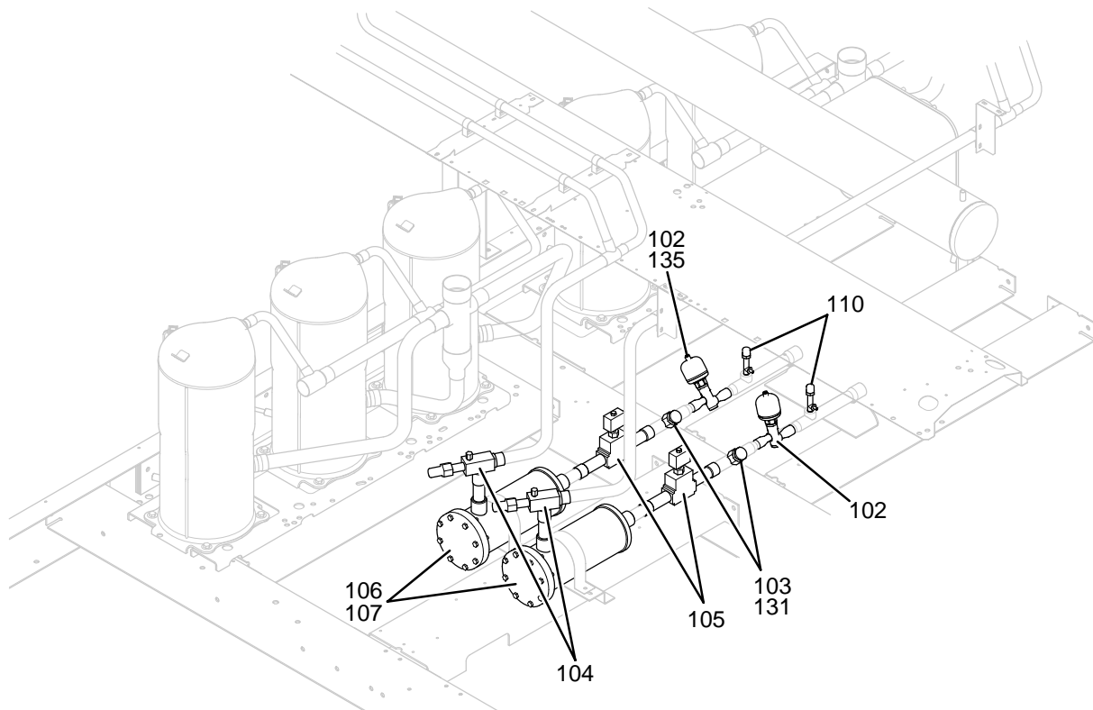
FIGURE 10 - SYSTEM PIPING (QTC3070T, QTC3075T, QTC3085T)
