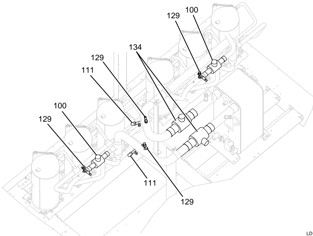
FIGURE 9 - SYSTEM PIPING (QTC3070T, QTC3075T, QTC3085T)
