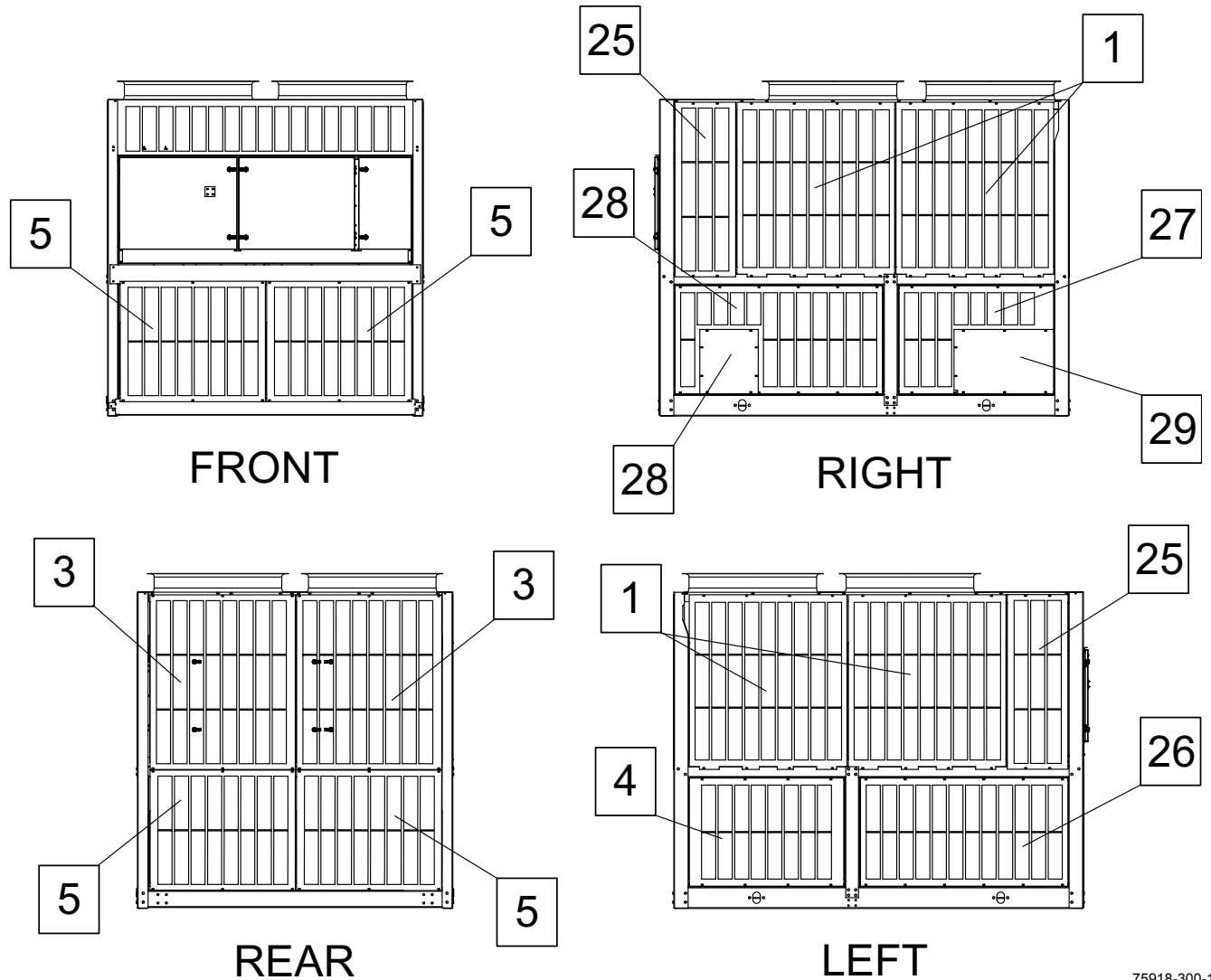
FIGURE 20 - LOUVERED ENCLOSURE
