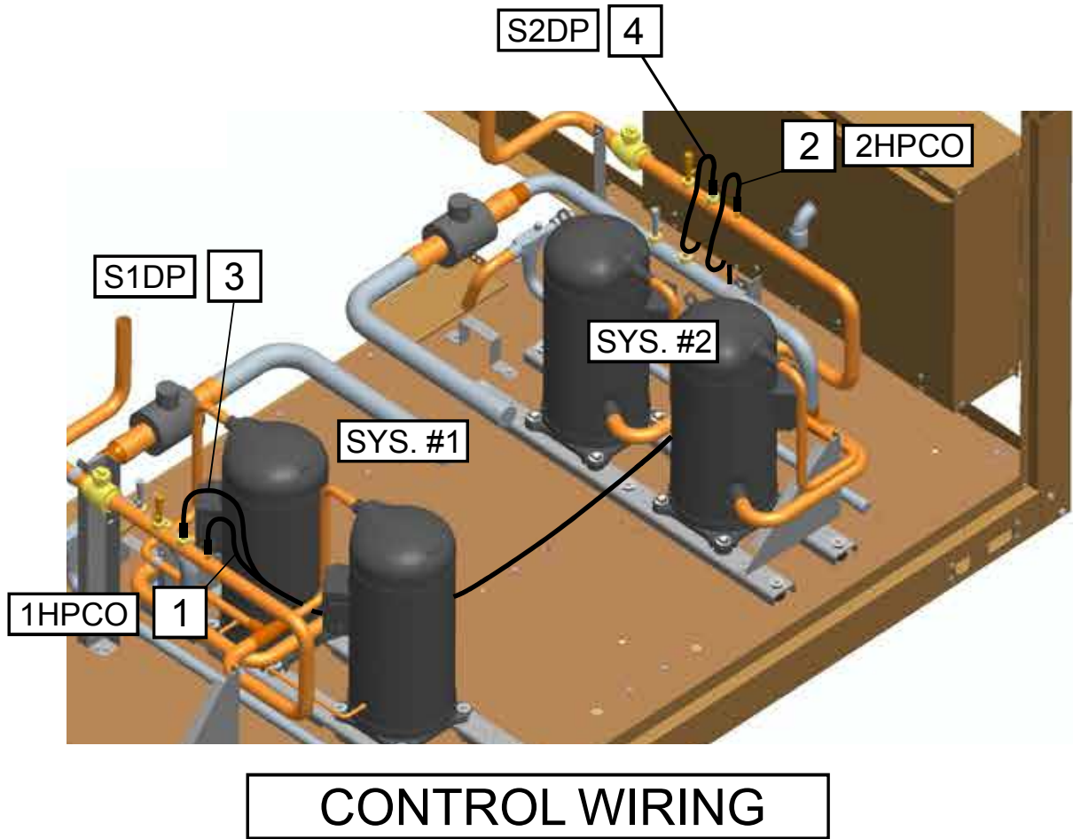
FIGURE 13 - CONTROL WIRING HARNESES
