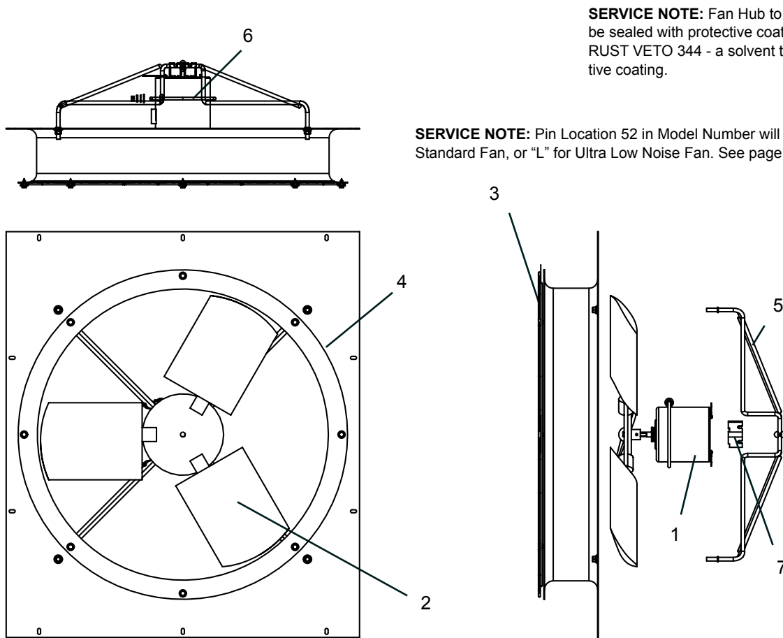
FIGURE 3 - FAN COMPONENTS - MODELS QCC2015C AND QCC2020C
