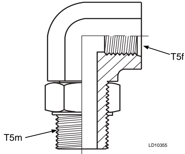
FIGURE 22 - STRAIGHT THREAD ELBOW
