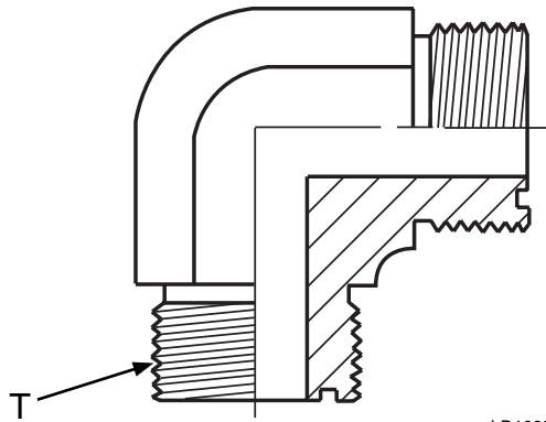
FIGURE 20 - ORFS ELBOW
