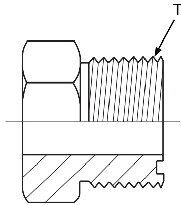
FIGURE 12 - ORFS TUBE END PLUG
