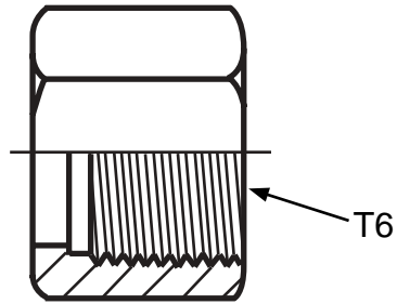
FIGURE 9 - O-RING FACE SEAL TUBE NUT
