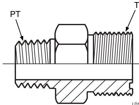
FIGURE 5 - ORFS X MALE PIPE CONNECTOR
