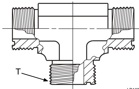
FIGURE 3 - ORFS UNION TEE
