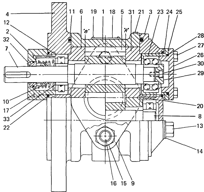
This pump used on units with 10" or 12" diameter oil coolers.
