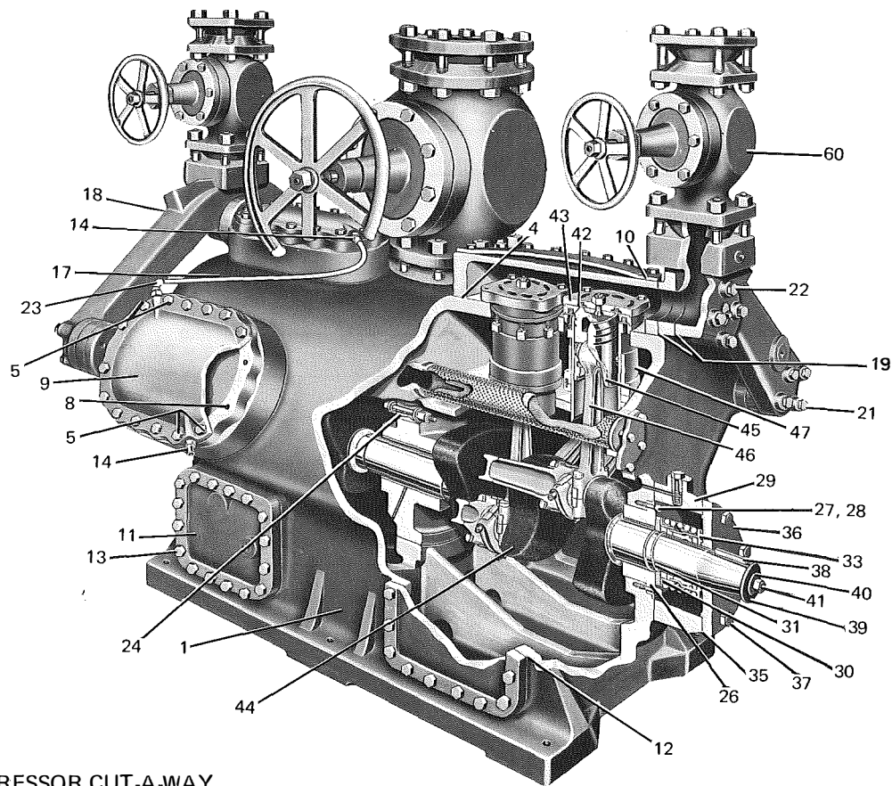
FIG. 1— COMPRESSOR CUT-A-WAY
