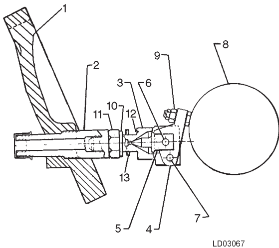
FIG. 11 – CRANKCASE FLOAT
