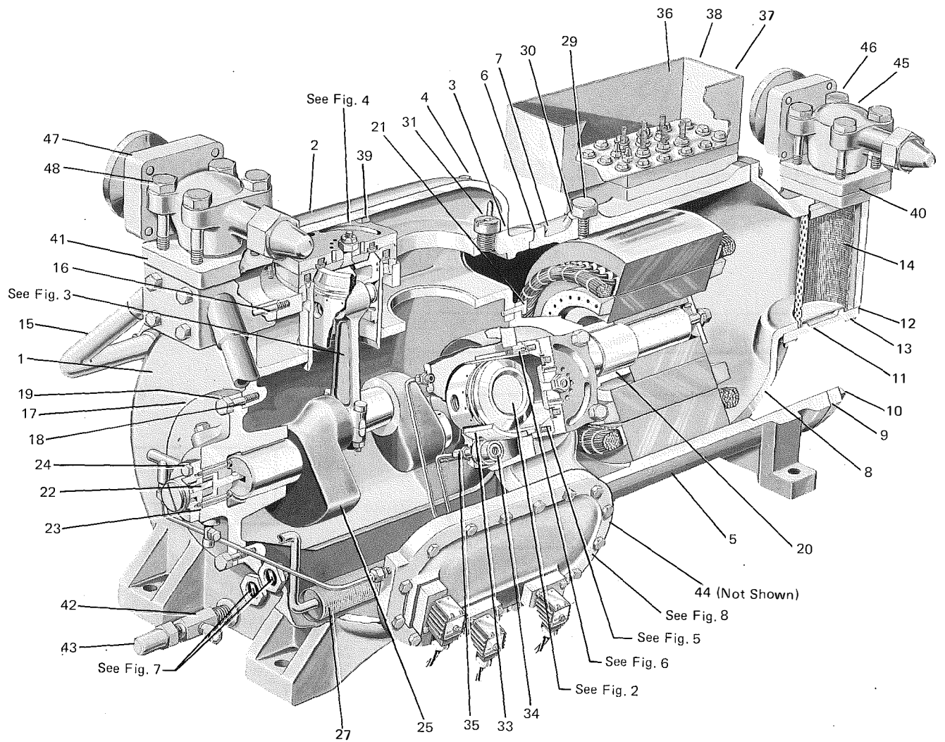
FIG. 1— COMPRESSOR CUT-A-WAY
