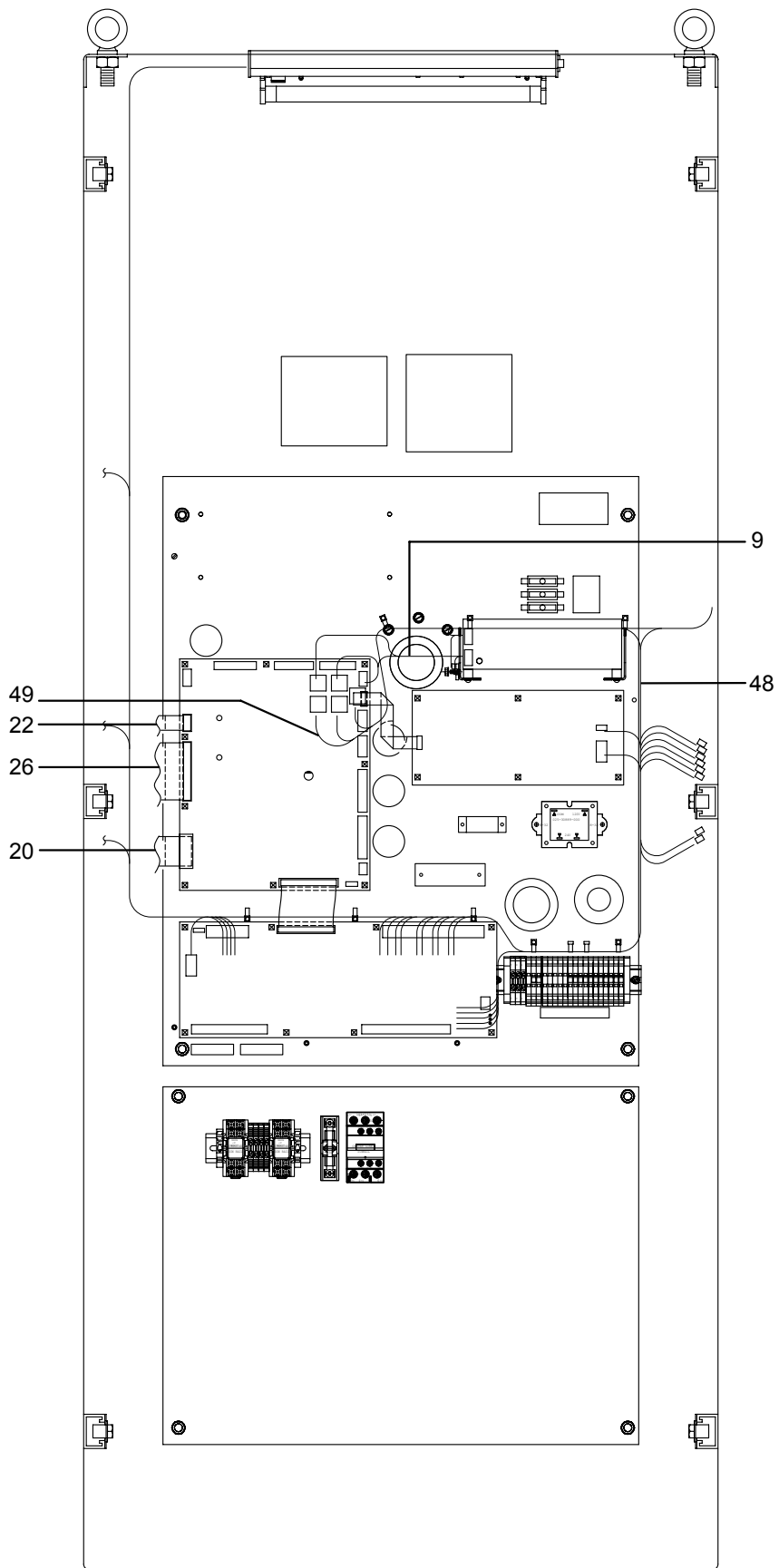
FIGURE 3 - INSIDE BACK PLATE WIRING
