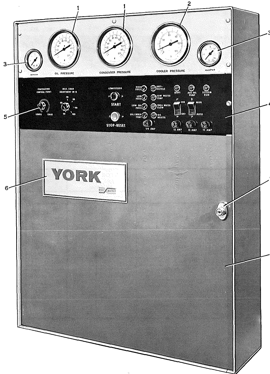
FIG. 1— TURBOMASTER CONTROL CENTER
