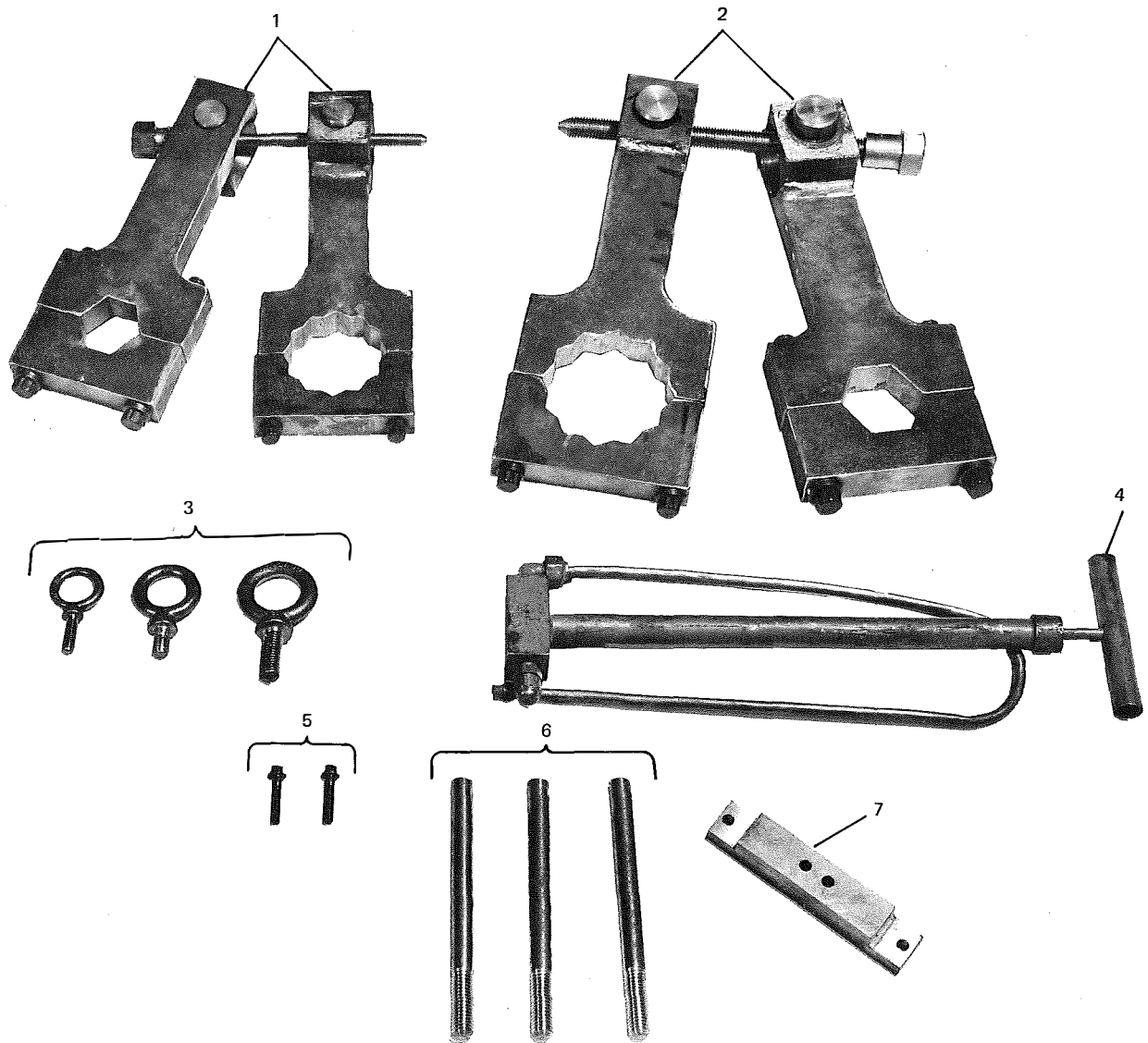
FIG. 14 – COMPRESSOR TOOLS FOR MODELS LKB65 & LKB73
