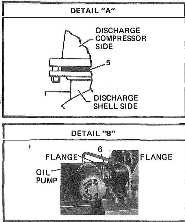
FIG. 4 – TURBOPAK SYSTEM DETAILS
