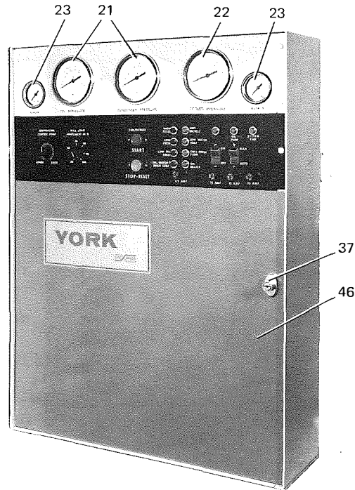
FIG. 25— PNEUMATIC CONTROL CENTER — DOOR CLOSED — Panel Part No.'s 366-17061-002, 366-17061-004
