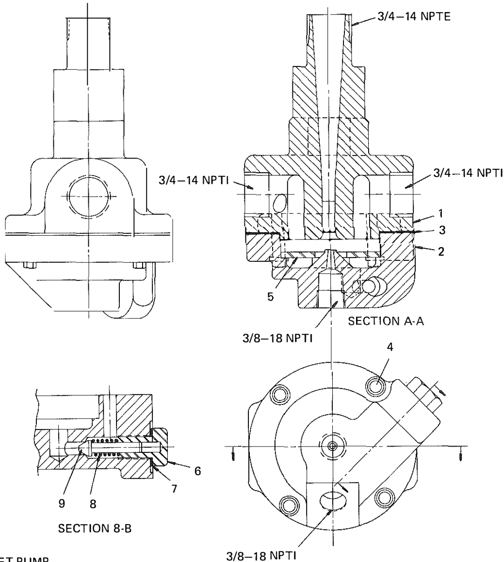
FIG. 46 — JET PUMP
