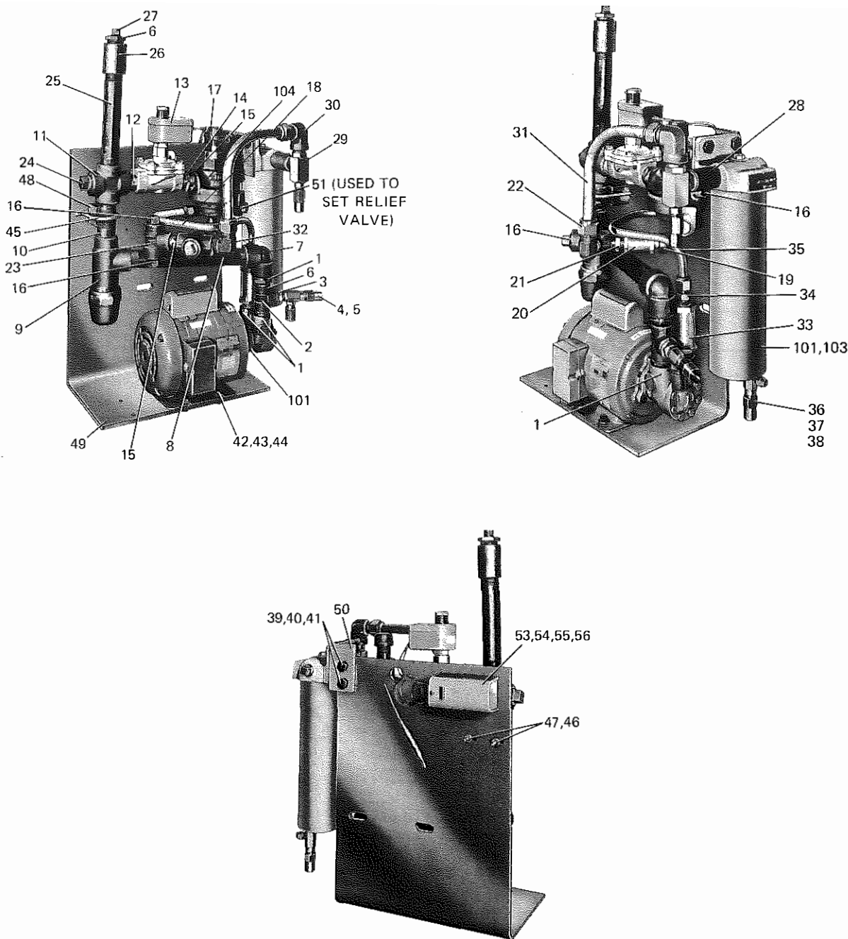
FIG. 45 – LUBE PACKAGE
