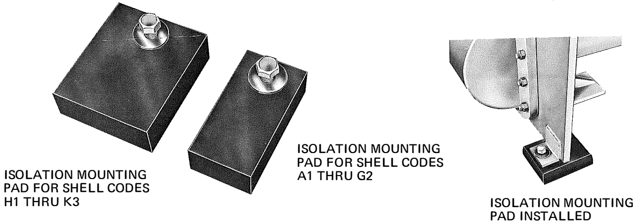
FIG. 3 — NEOPRENE ISOLATOR INSTALLATION
