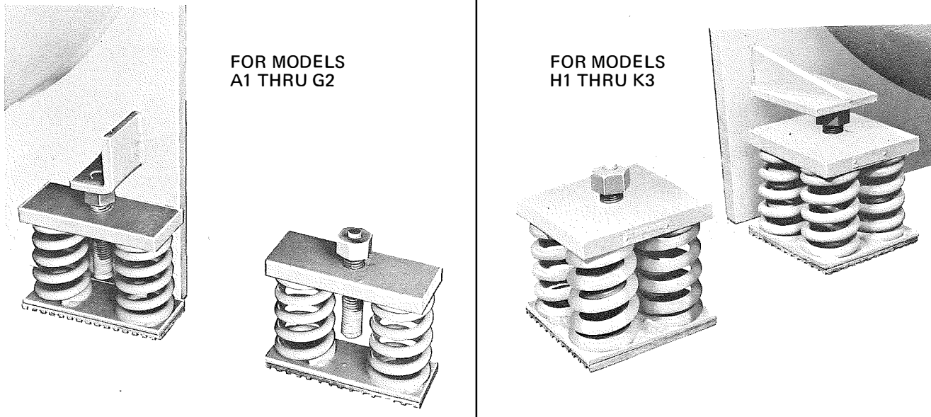
FIG. 4 — SPRING ISOLATORS
