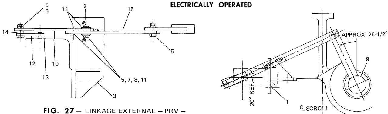
FIG. 27 - LINKAGE EXTERNAL - PRV - ELECTRICALLY OPERATED
