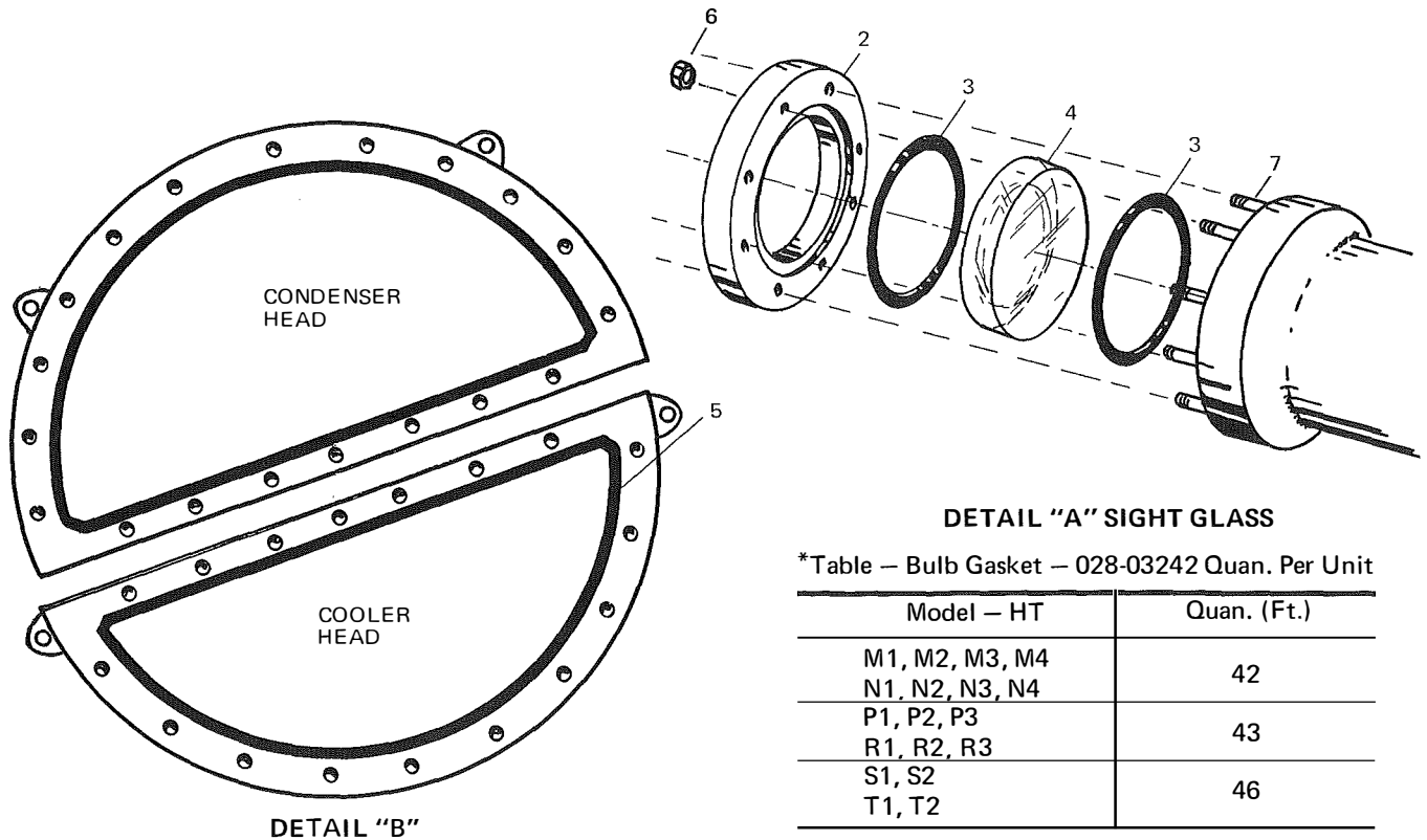
FIG. 1— COOLER—CONDENSER SHELL
