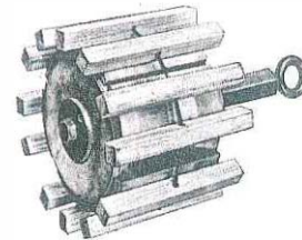
FIG. 25 — HERMETIC MOTOR EXPANDING MANDREL
