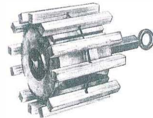
FIG. 25 — HERMETIC MOTOR EXPANDING MANDREL MANDREL PART NUMBERS
