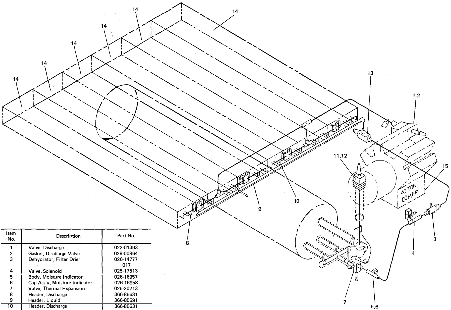
FIG. 9— REFRIGERANT PIPING — LCHA35
