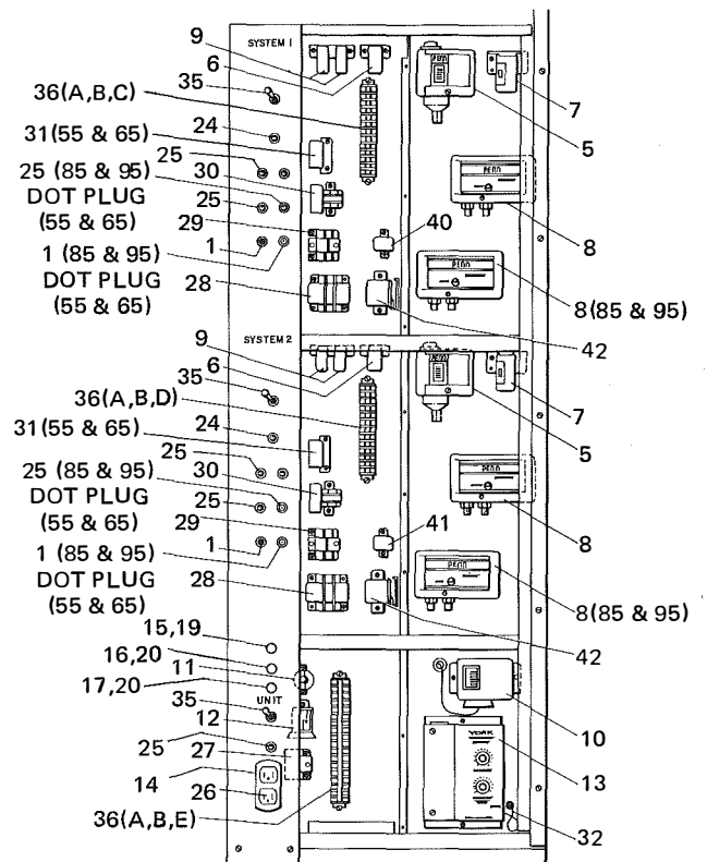
FIG. 4 - CONTROL SECTION
