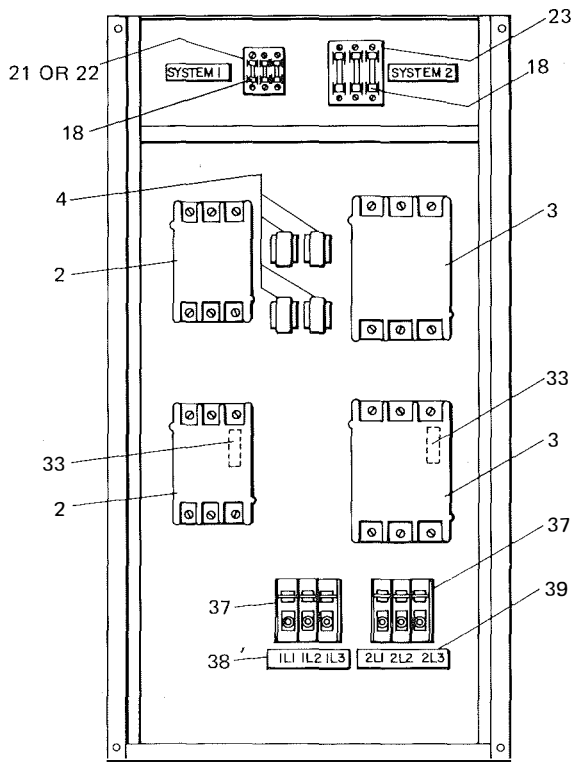
FIG. 3 - POWER SECTION
