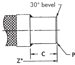
Type W Butt-weld end
