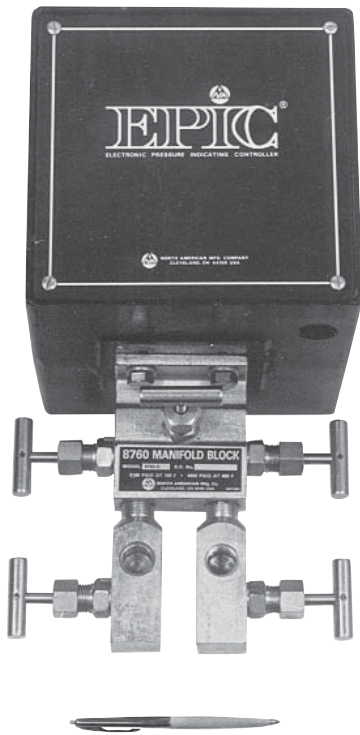
8351A-T Transmitter with 8760-D Manifold Block mounted.
